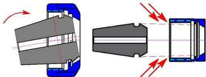
Hex, EType & RD Eccentric Design
