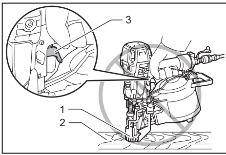
► 1. Contact element 2. Workpiece 3. Trigger (not pulled)
