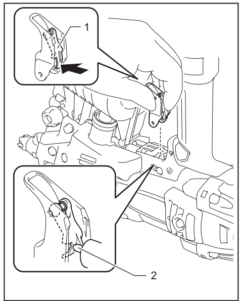
► 1. Hinged part 2. Rod of the valve
