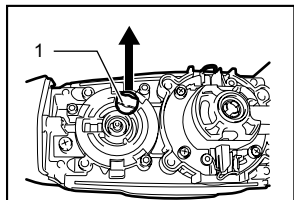
1. Grease cap
